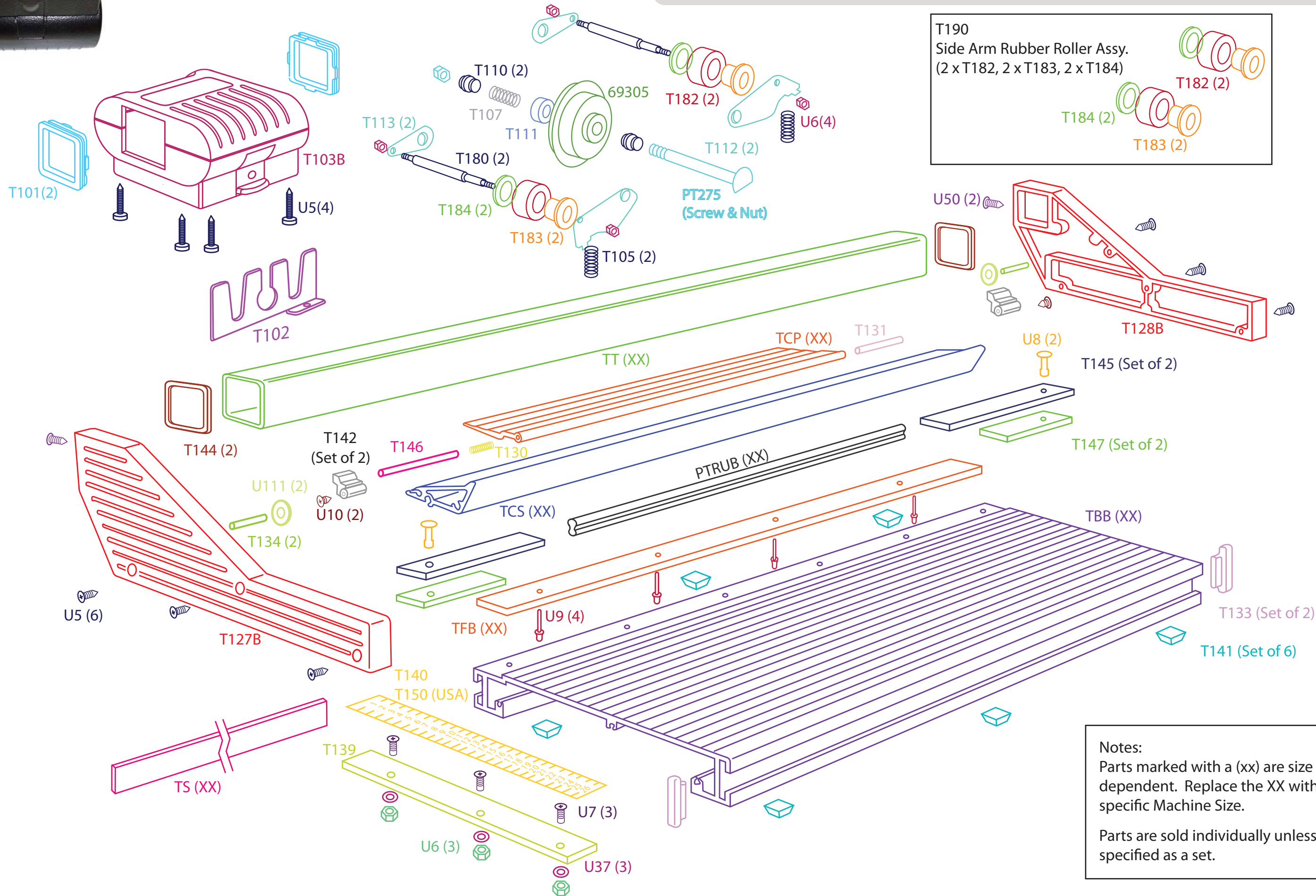
T100A (Complete Cutting Head)
